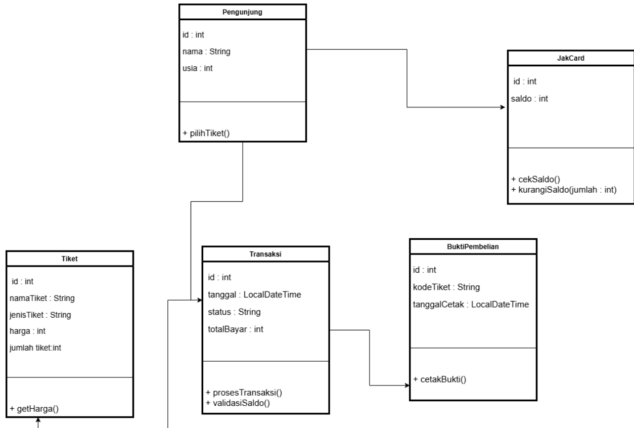
Class Diagram
