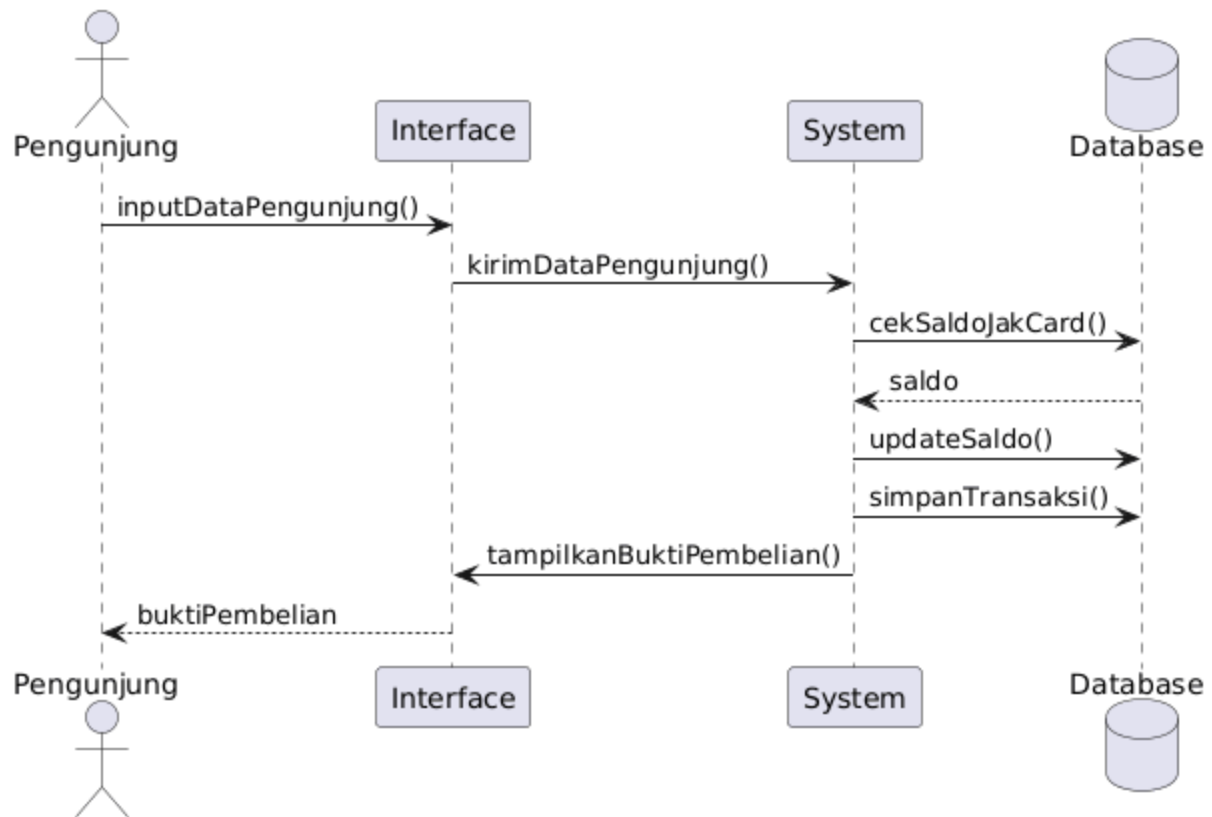
Sequence diagram
