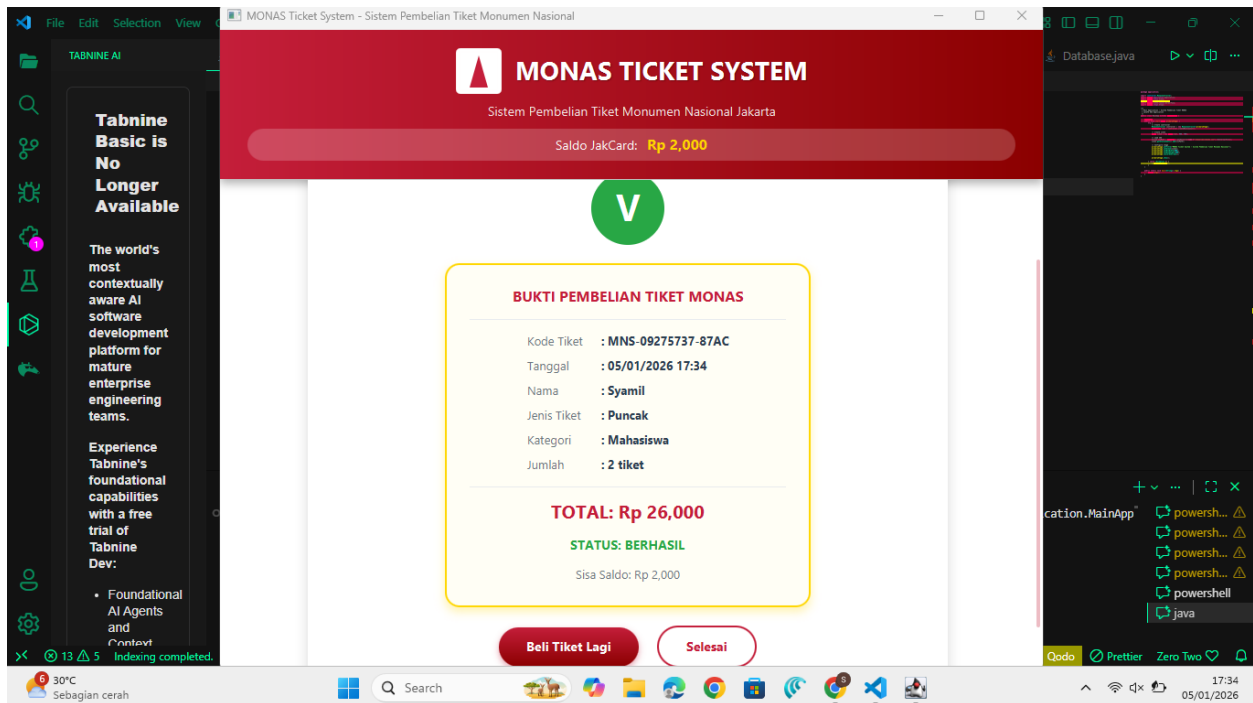
ScreenJava gui
